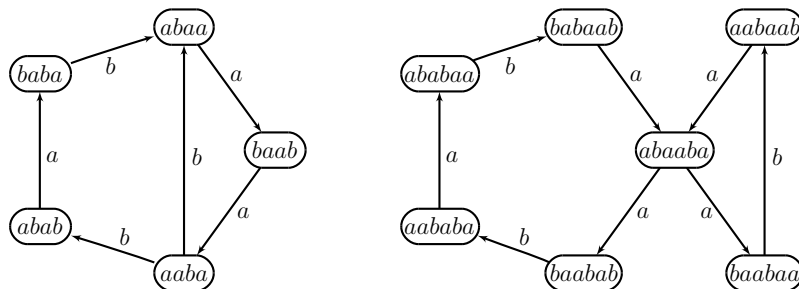
FIGURE 1. Centrally labeled Rauzy graphs of order 4 and 6 associated to the Fibonacci substitution [ab, a] .
