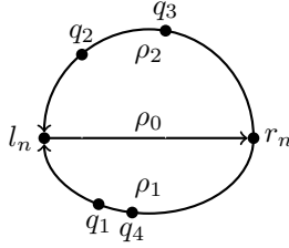
FIGURE 6. Diagram for the proof of Theorem 4.7
