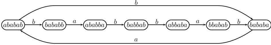
FIGURE 2. Rauzy graph associated to \varphi = [bababbaba, ba] .
