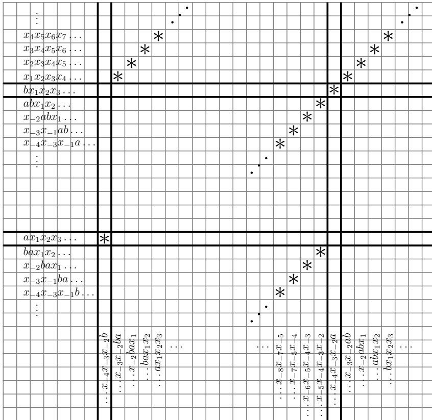
FIGURE 7. Picture representing a portion of \mathcal{JM}(\mathcal{X}) when \mathcal{X} is Sturmian. Rows represent \mathcal{R} -classes, columns represent \mathcal{L} -classes, and stars indicate \mathcal{H} -classes with idempotents. In each row/column is indicated the nonnegative/negative ray parameterizing it.
