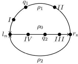
FIGURE 5. Positions I to IV for vertex p in the proof of Lemma 4.6.
