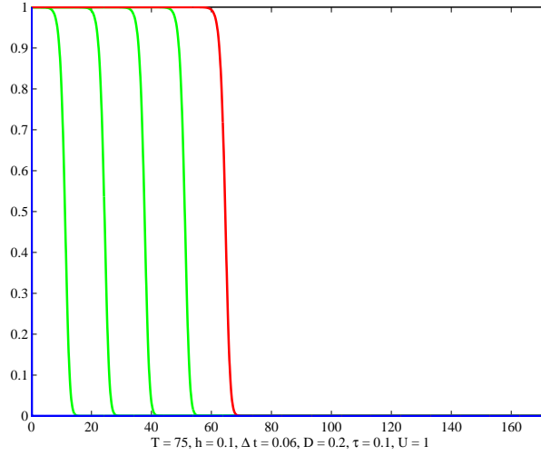
FIGURE 7. Numerical solution obtained using Method D_{n+1}R_n - stable behaviour.
