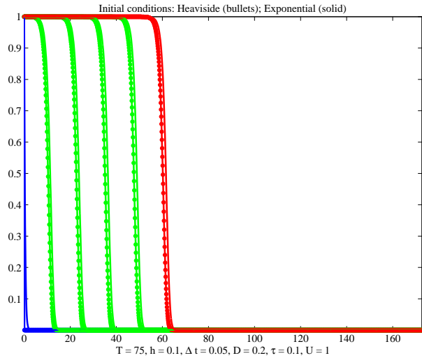
FIGURE 5. Traveling waves for u_0(x) = H(x) and u_0(x) = e^{m^*(-x+c_+(m^*)t)} .
