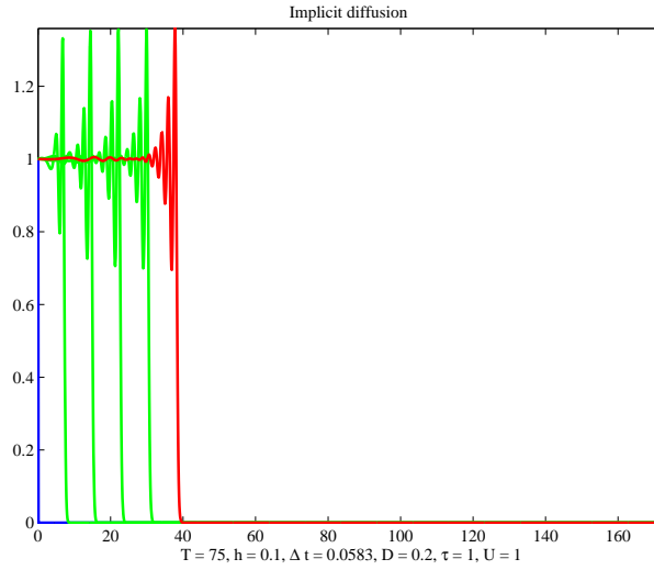
FIGURE 8. Numerical solutions obtained using Methods D_{n+1}R_n - oscillatory behaviour.
