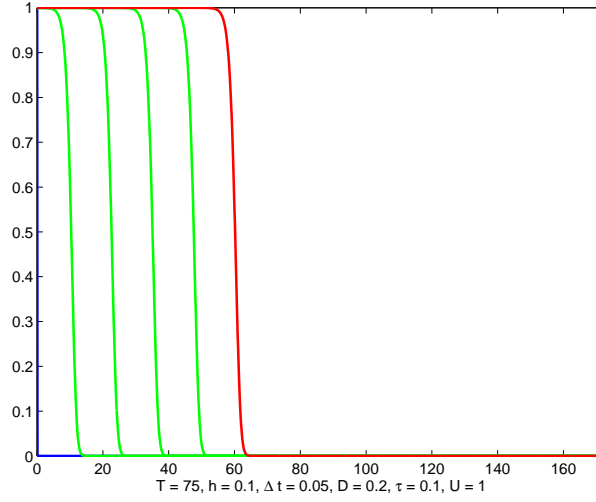
FIGURE 2. Numerical solutions obtained by Method D_n R_n - stable behaviour.
