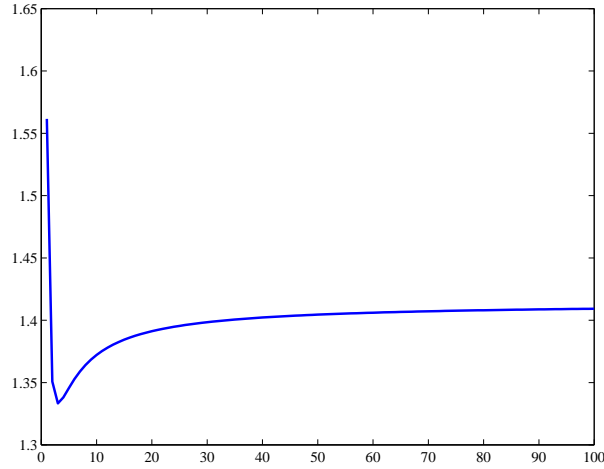
FIGURE 4. The graph of c_+(m) .
