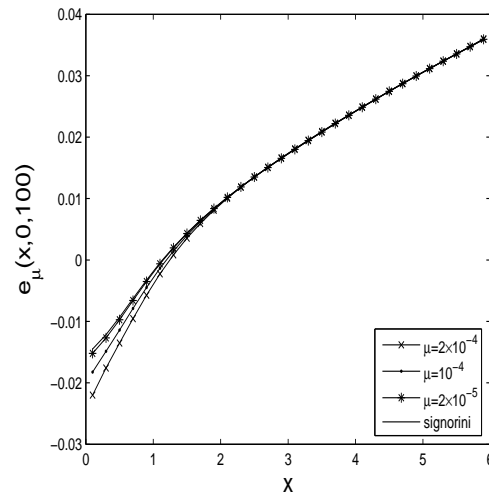
FIGURE 9. Example 2D: Bone remodeling function, on the contact boundary, depending on \mu .
