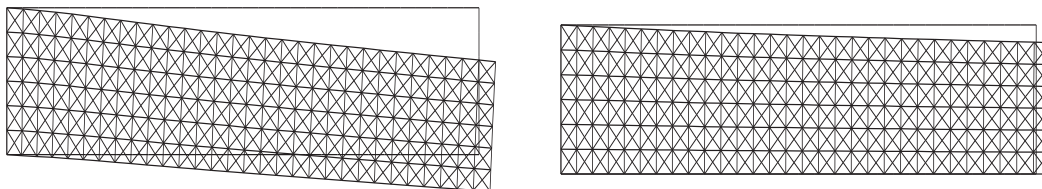
FIGURE 6. Example 2D: Deformed rectangle in contact with a deformable obstacle (left) and with a rigid one (right).
