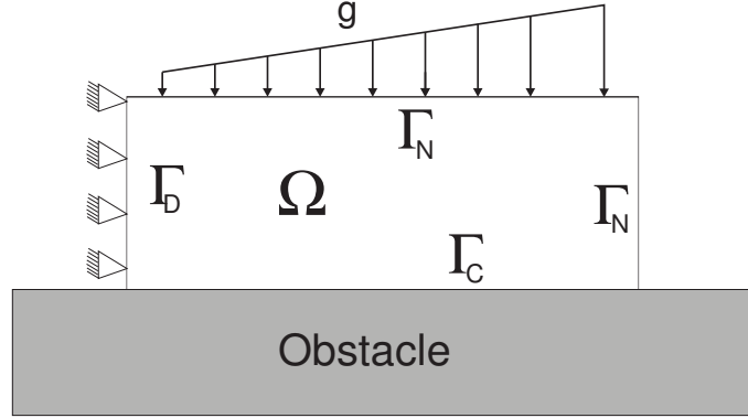
FIGURE 5. Example 2D: A rectangle in contact with an obstacle.
