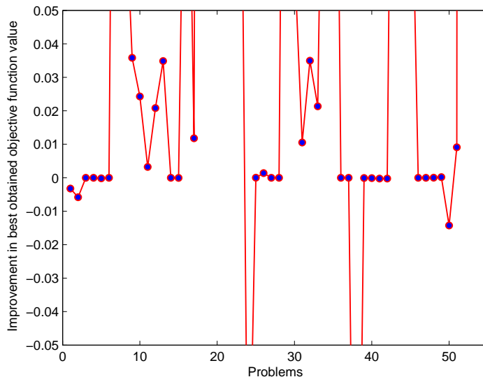
FIGURE 1. Difference in best function values obtained for a set of smooth problems. Positive (resp. negative) values indicate better performance of Ssid-psm /Algorithm 4.1 (resp. of sid-psm ).
