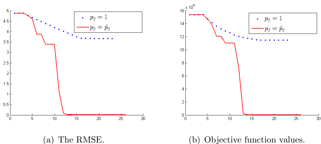
FIGURE 3. Results of one run of Algorithm 7.1 when using probabilities p_j = 1 (dotted line) and p_j = \tilde{p}_j (solid line).
