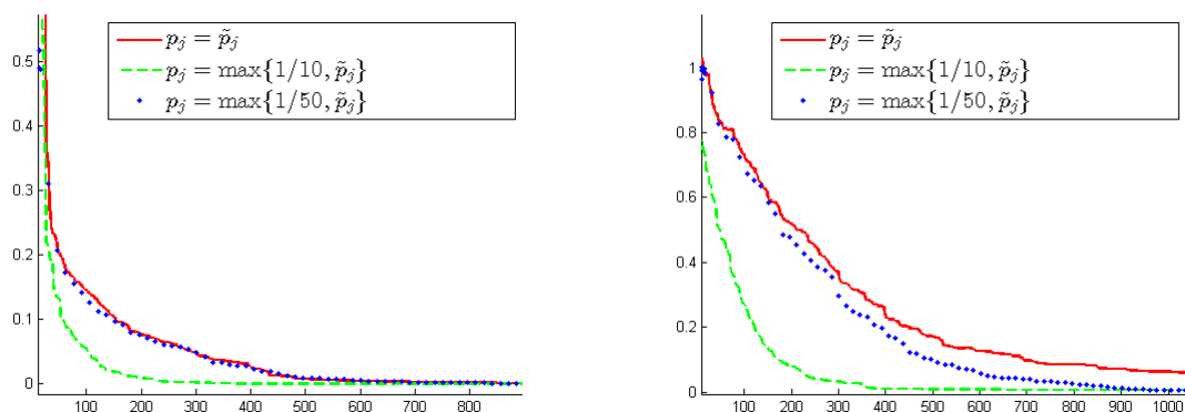
(a) Average of function values.
