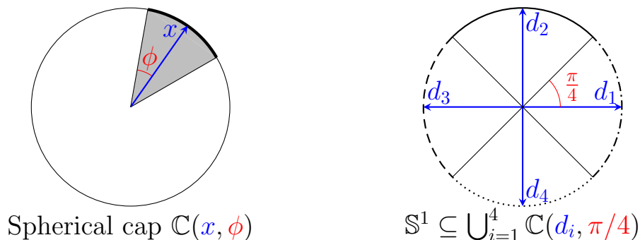
FIGURE 2. The thick arc of the left picture represents a spherical cap in \mathbb{R}^2 . The right picture depicts the covering of the unit sphere given in Lemma 4.1 for D_{\oplus} when n = 2 .
