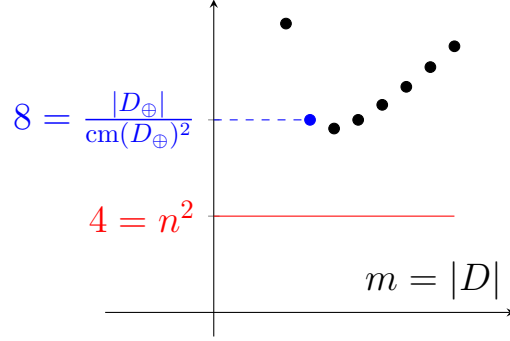
FIGURE 1. Illustration of inequality (8) in \mathbb{R}^2 for PSSs making uniform adjacent angles. The plot depicts the values of |D|/\text{cm}(D)^2 for |D| = 3, 4, \dots, 10 .
