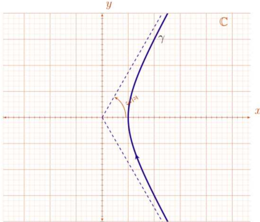
Branch of hiperbola 3x^2 - y^2 = 3
