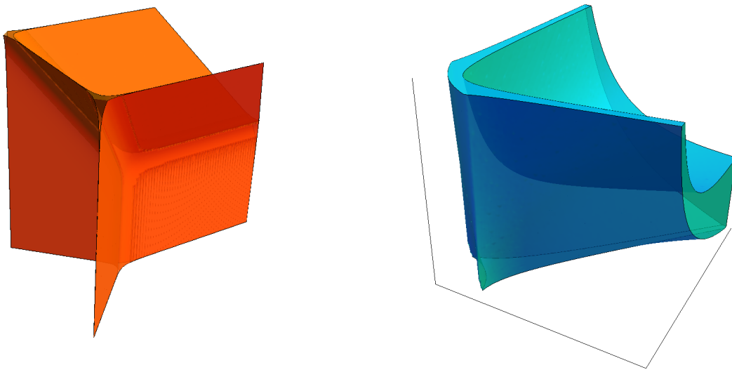
FIGURE 2. \mathcal{A}(V) and \mathcal{A}_{\text{alg}}(V) of a determinantal variety.
