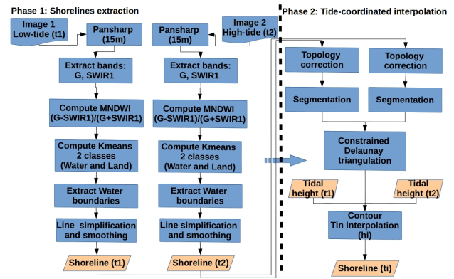
Figure 2: Methodology flowchart
