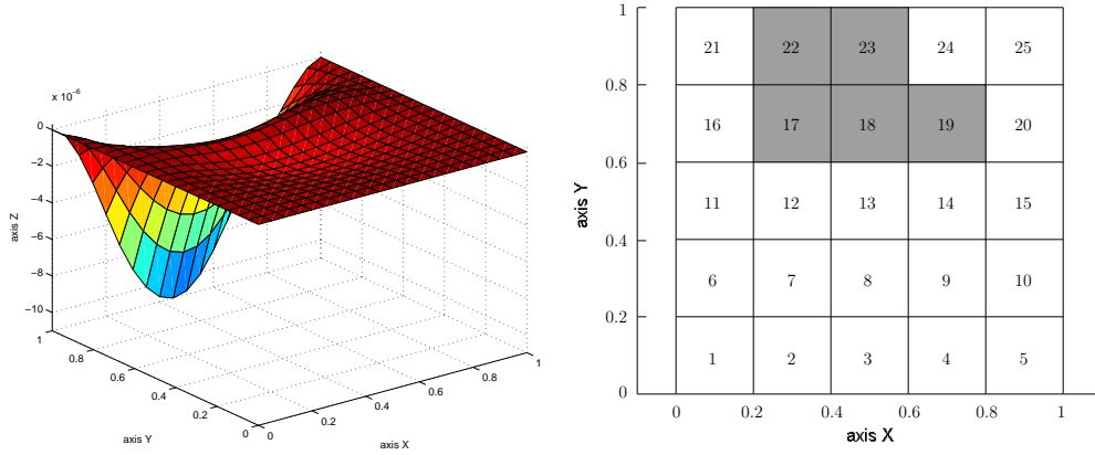
Figure 5. Actuator optimization problem: transverse displacement of the plate's middle plane for BC = 2 (left plot) and corresponding optimal position pe=[17,18,19,22,23] of the regions where the non-zero electric potential difference is applied (right plot).
