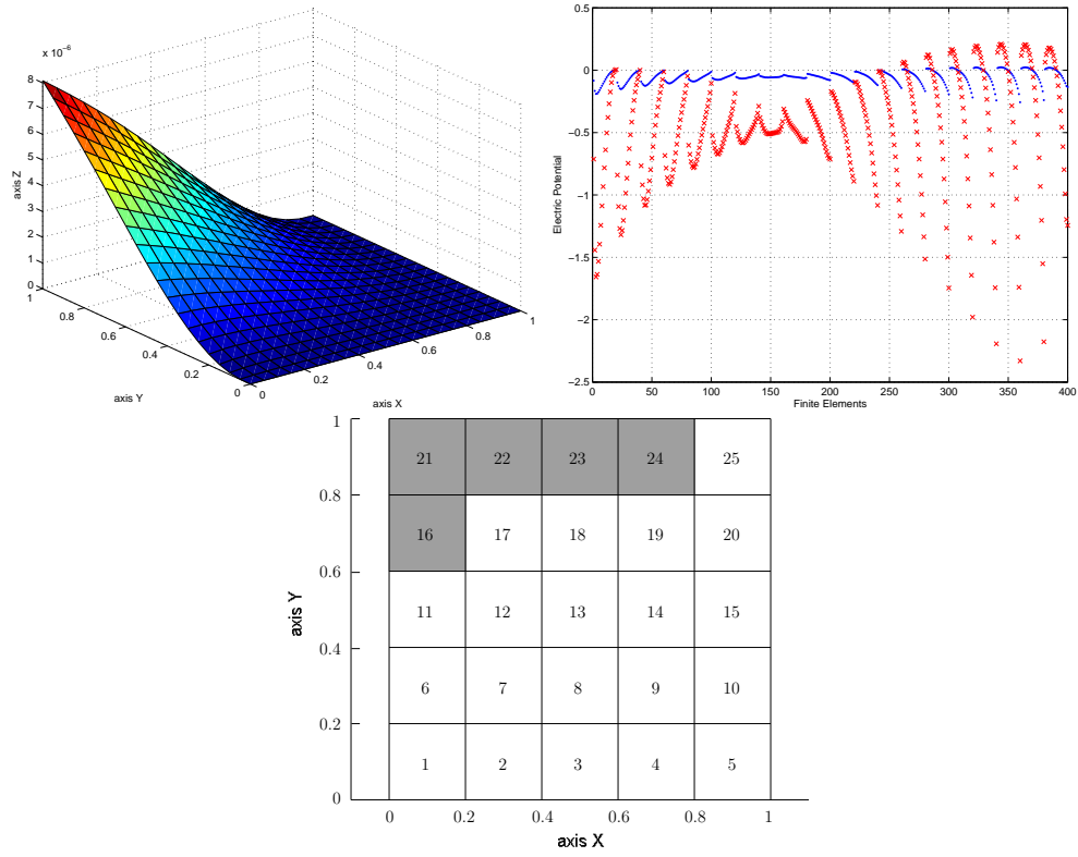
Figure 11. Sensor optimization problem: transverse displacement of the plate's middle plane for BC = 4 (upper left plot), electric potentials (cross mark - \varphi|_{\omega^e \times \{z_1\}} on lamina 1, and, dotted - \varphi|_{\omega^e \times \{z_2\}} on lamina 2) (upper right plot) and corresponding optimal position pe=[16,21,22,23,24] of the regions where the non-zero mechanical forces are applied (lower plot).
