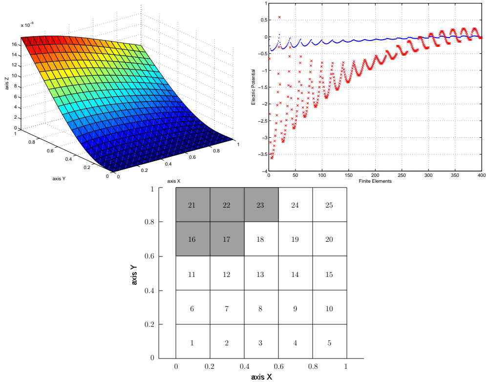
Figure 8. Sensor optimization problem: transverse displacement of the plate's middle plane for BC = 1 (upper left plot), electric potentials (cross mark - \varphi|_{\omega^e \times \{z_1\}} on lamina 1 and dotted - \varphi|_{\omega^e \times \{z_2\}} on lamina 2) (upper right plot) and corresponding optimal position pe=[16,17,21,22,23] of the regions where the non-zero mechanical forces are applied (lower plot).
