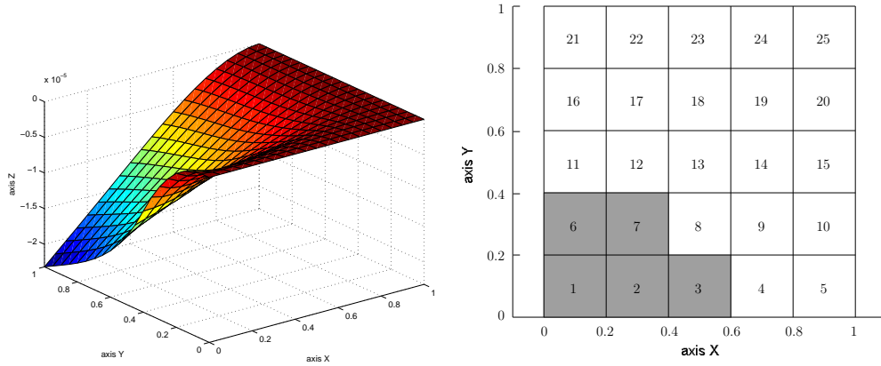
Figure 7. Actuator optimization problem: transverse displacement of the plate's middle plane for BC = 4 (left plot) and corresponding optimal position pe=[1,2,3,6,7] of the regions where the non-zero electric potential difference is applied (right plot).
