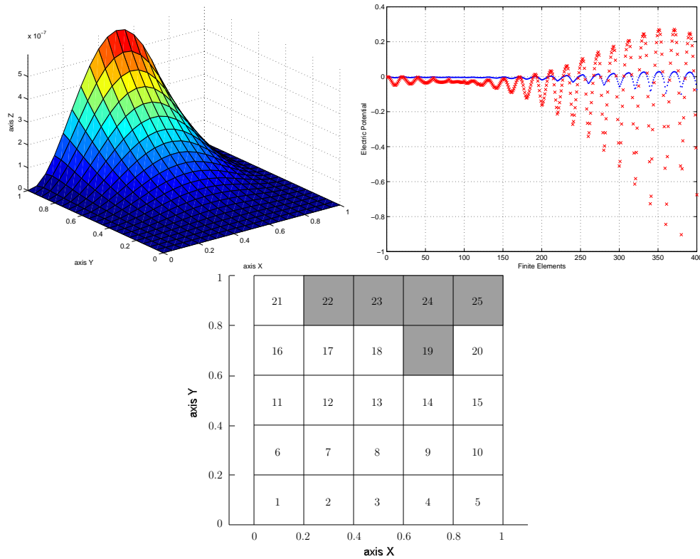
Figure 9. Sensor optimization problem: transverse displacement of the plate's middle plane for BC = 2 (upper left plot), electric potentials (cross mark - \varphi|_{\omega^e \times \{z_1\}} on lamina 1 and dotted - \varphi|_{\omega^e \times \{z_2\}} on lamina 2) (upper right plot), and corresponding optimal position pe=[19,22,23,24,25] of the regions where the non-zero mechanical forces are applied (lower plot).
