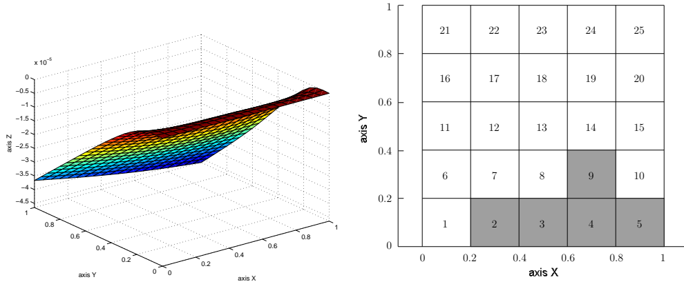
Figure 4. Actuator optimization problem: transverse displacement of the plate's middle plane for BC = 1 (left plot) and corresponding optimal position pe=[2,3,4,5,9] of the regions where the non-zero electric potential difference is applied (right plot).
