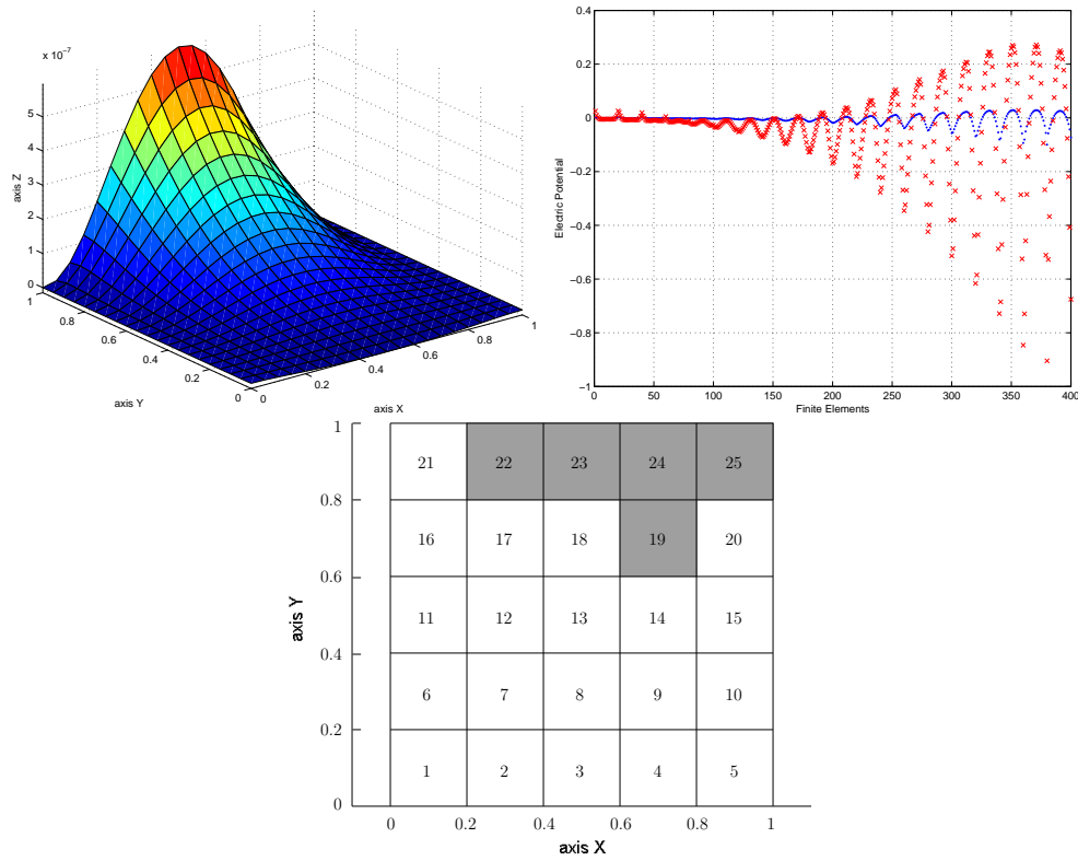
Figure 10. Sensor optimization problem: transverse displacement of the plate's middle plane for BC = 3 (upper left plot), electric potentials (cross mark - \varphi|_{\omega^e \times \{z_1\}} on lamina 1, and, dotted - \varphi|_{\omega^e \times \{z_2\}} on lamina 2) (upper right plot) and corresponding optimal position pe=[19,22,23,24,25] of the regions where the non-zero mechanical forces are applied (lower plot).
