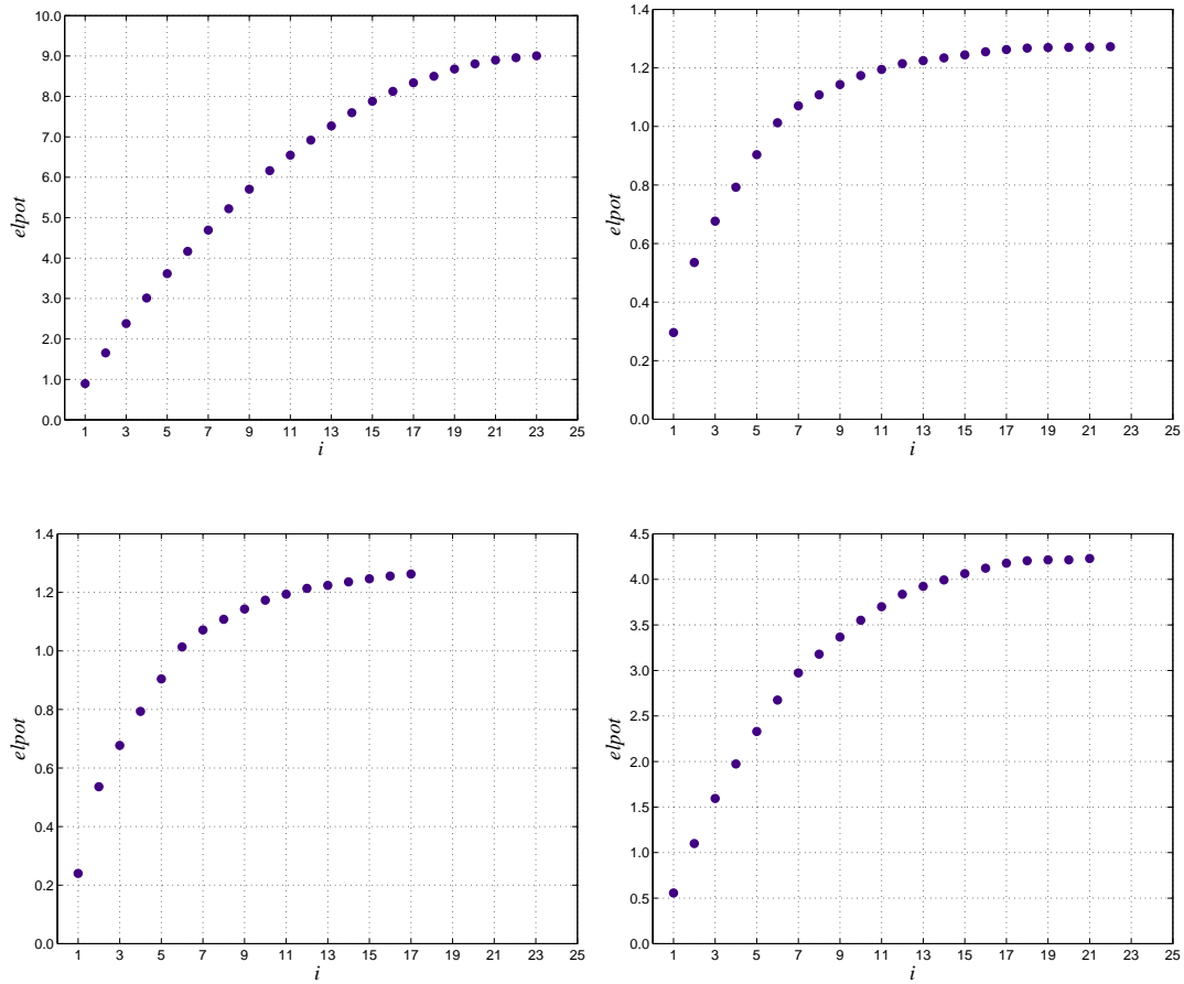
Figure 3. Pareto curves: maximal electric potential elpot versus number of regions i (where the mechanical loads are applied) for the sensor multi-objective problem for BC = 1 (upper left plot), BC = 2 (upper right plot), BC = 3 (lower left plot) and BC = 4 (lower right plot).
