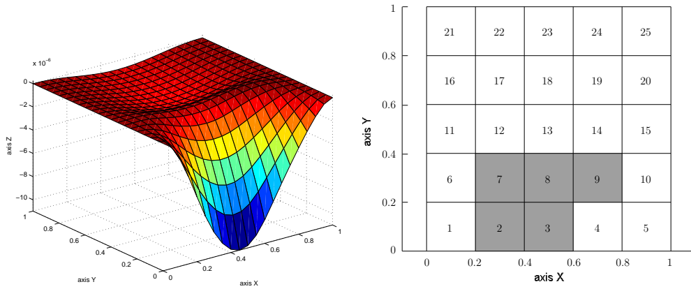
Figure 6. Actuator optimization problem: transverse displacement of the plate's middle plane for BC = 3 (left plot) and corresponding optimal position pe=[2,3,7,8,9] of the regions where the non-zero electric potential difference is applied (right plot).
