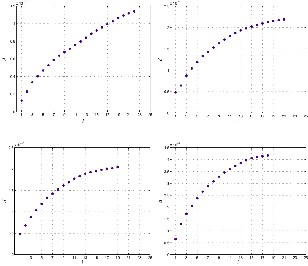
Figure 2. Pareto curves: maximal displacement d versus number of regions i (where the electric potential difference \varphi_0^+ - \varphi_0^- is applied) for the actuator multi-objective problem for BC = 1 (upper left plot), BC = 2 (upper right plot), BC = 3 (lower left plot) and BC = 4 (lower right plot).
