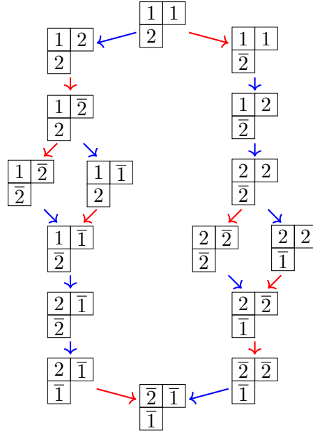
FIGURE 1. The type C_2 crystal graph \mathcal{KN}((2,1),2) containing the A_1 crystal \mathcal{SSYT}((2,1),2) , consisting of the two top left most tableaux, as a subcrystal. The type C_2 lowering crystal operators are f_1 , \rightarrow , and f_2 , \rightarrow .
