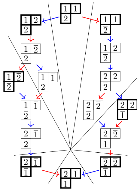
FIGURE 4. The partition of the C_2 crystal graph \mathfrak{B}(2, 1) into |B_2(2, 1)| = 8 Demazure atom crystals .
